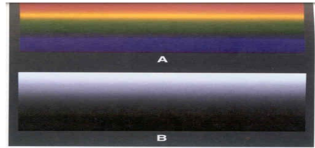
Plate 3.9 A comparison of rainbows defined by wavelength versus intensity. Both figures show a rainbow defined by a single physical continuum: wavelength in A and intensity in B. Nevertheless, the wavelength rainbow has a distinctly banded appearance that is not present in the intensity rainbow. These bands may reflect the categorical structure of perceived color.
